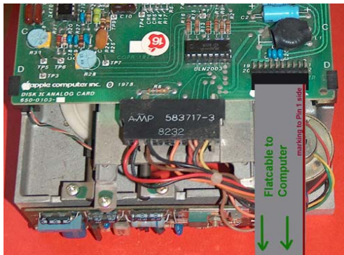
Rearview of the drive
