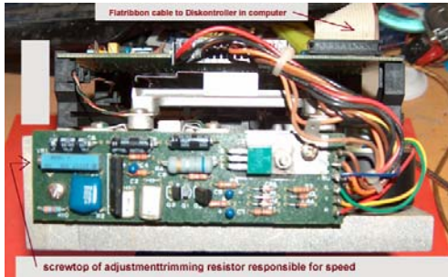
Rearview of the drive
